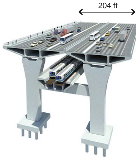
4. Stacked Option
